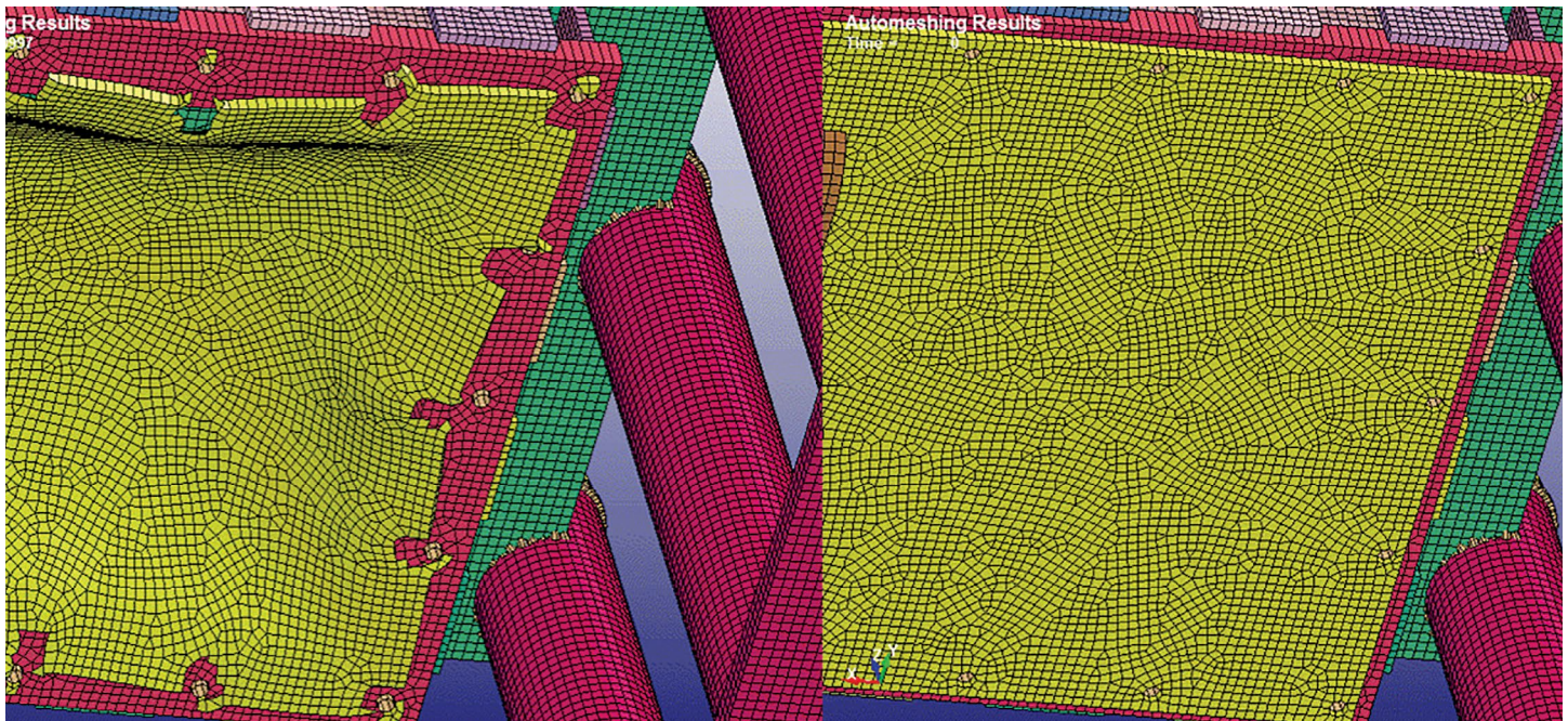
This computation shows that strong bolts can tear a test panel during loading (left), while weak bolts will break (right).
