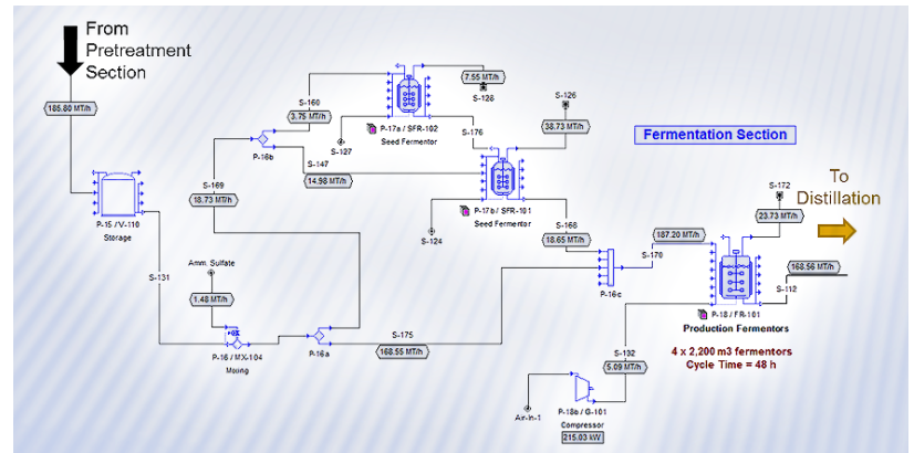
Simulating the corn stover to ethanol process
